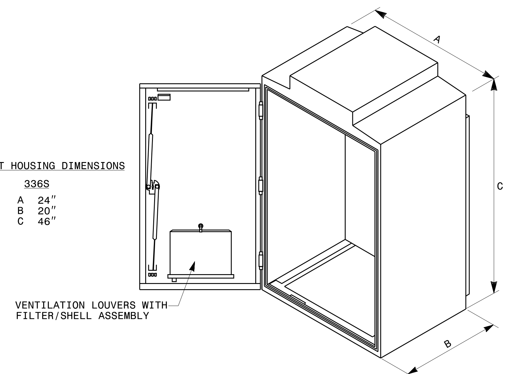
EQUIPMENT CABINET SIZES
